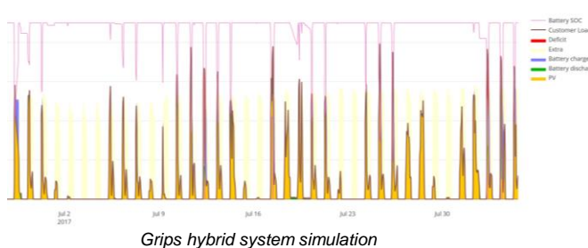
Grips hybrid system simulation
